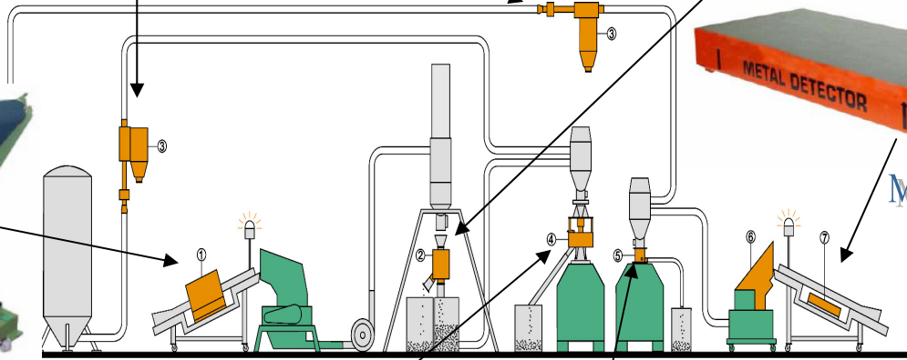
Metal Detector DLS
